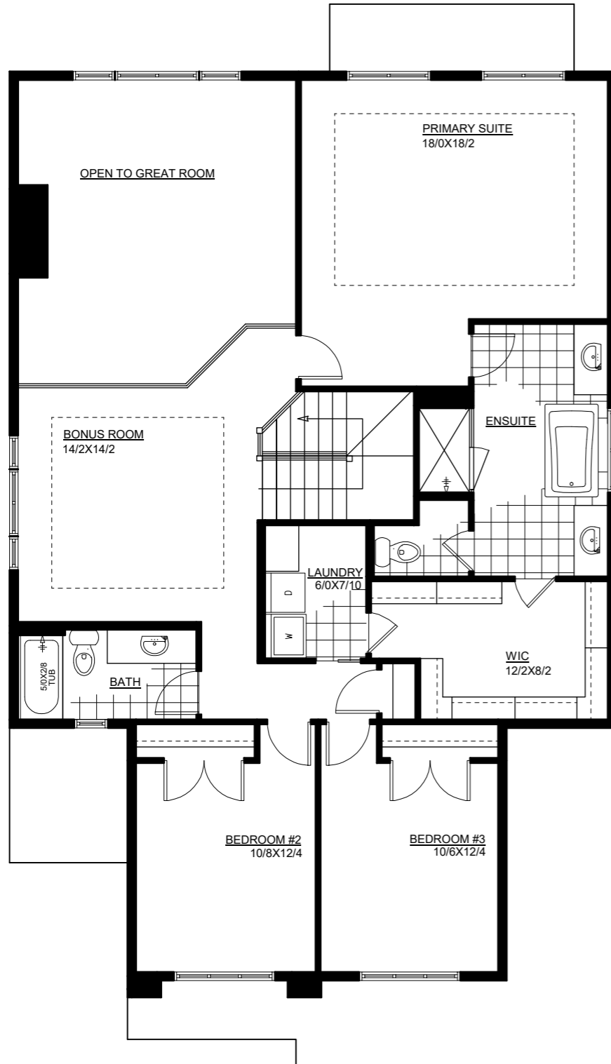
UPPER FLOOR PLAN 1392.0 sq.ft.
