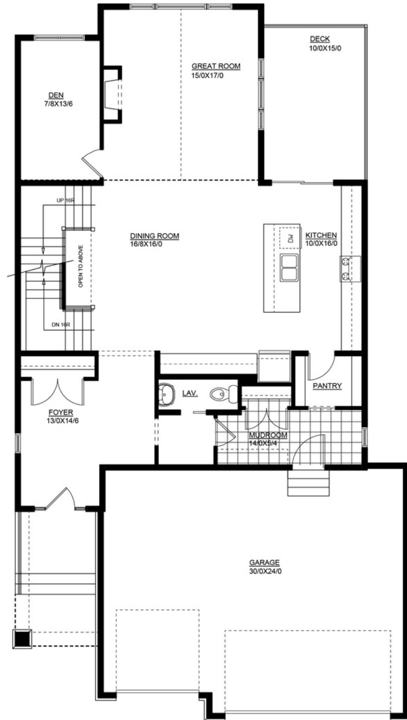
Main Floor | 1370 sqft
