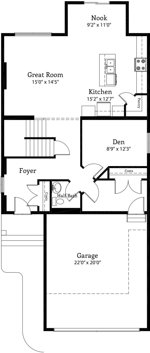
MAIN FLOOR | 1024 sq. ft.
