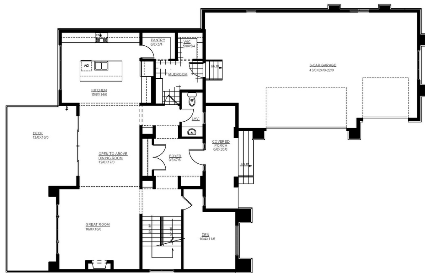
Main Floor - 1425 sqft
