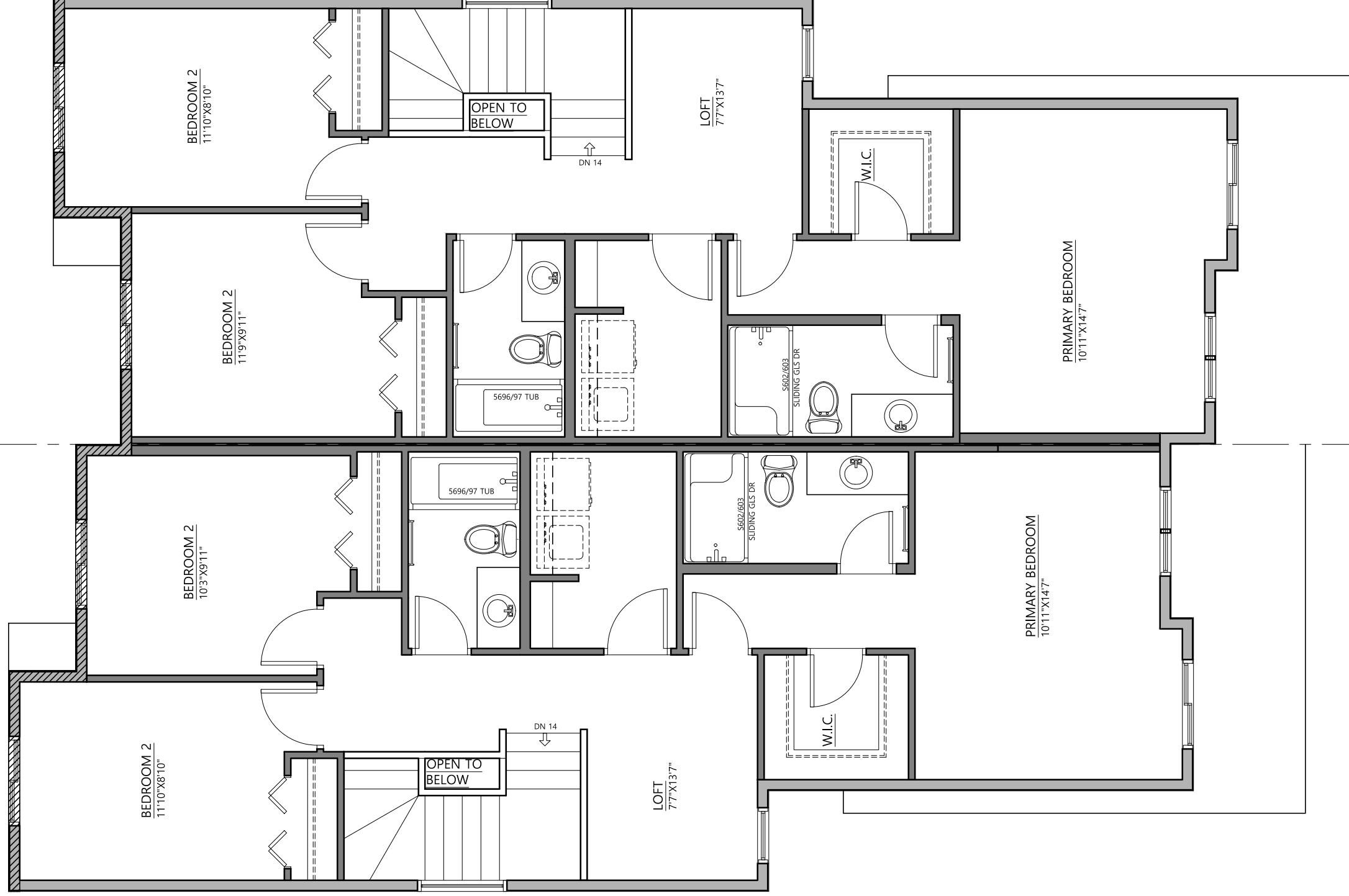
(ONYX) 8'1" UPPER FLOOR PLAN
