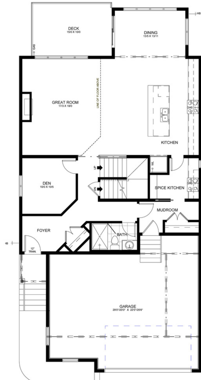
Main Floor - 1348 sqft
