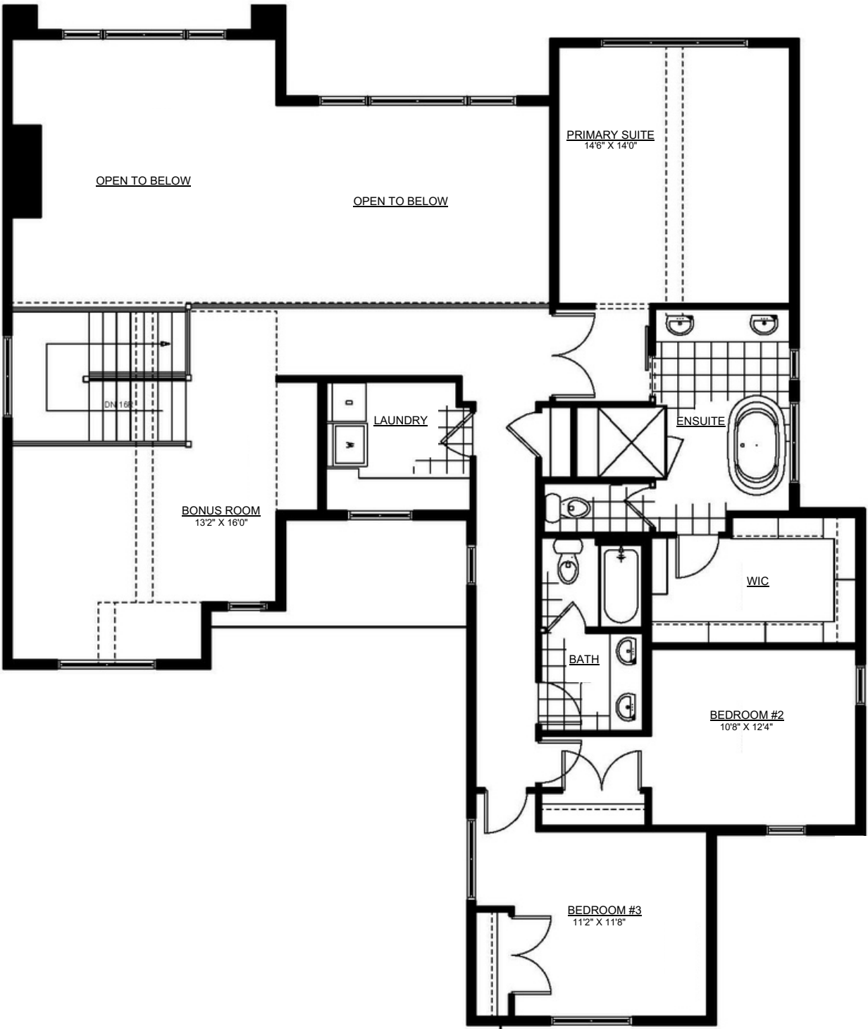
Upper Floor | 1572 sqft
