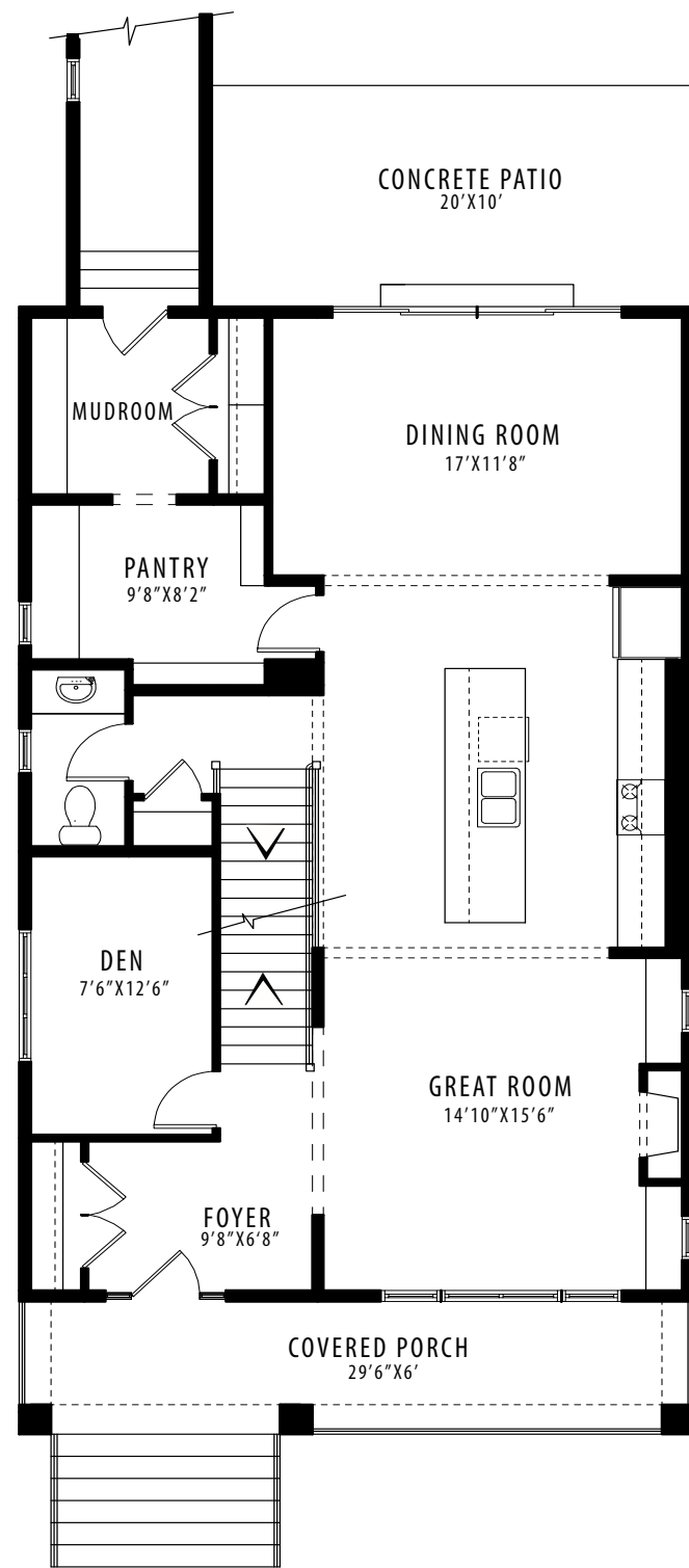
MAIN FLOOR | 1260 SQ FT
