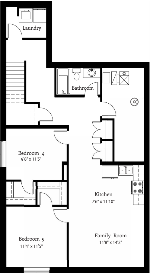
LEGAL SUITE | 919 SQ.FT
