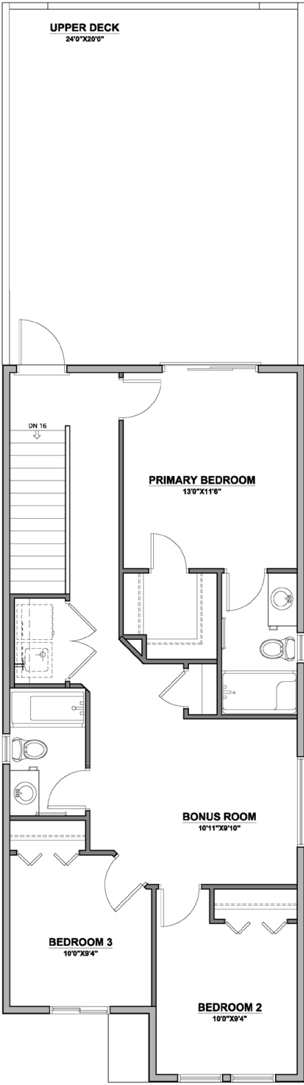
Upper Floor | 861 sq.ft.
