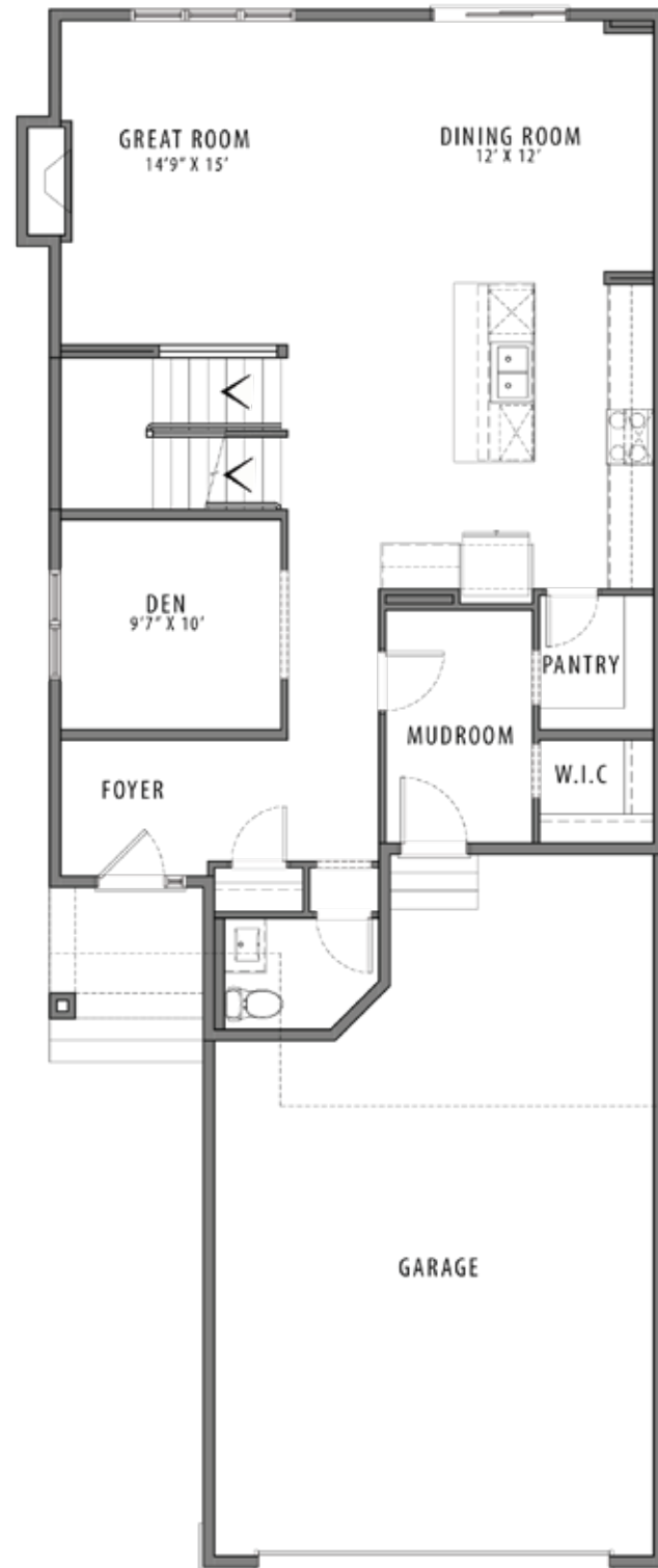
MAIN FLOOR | 1158 SQ FT
