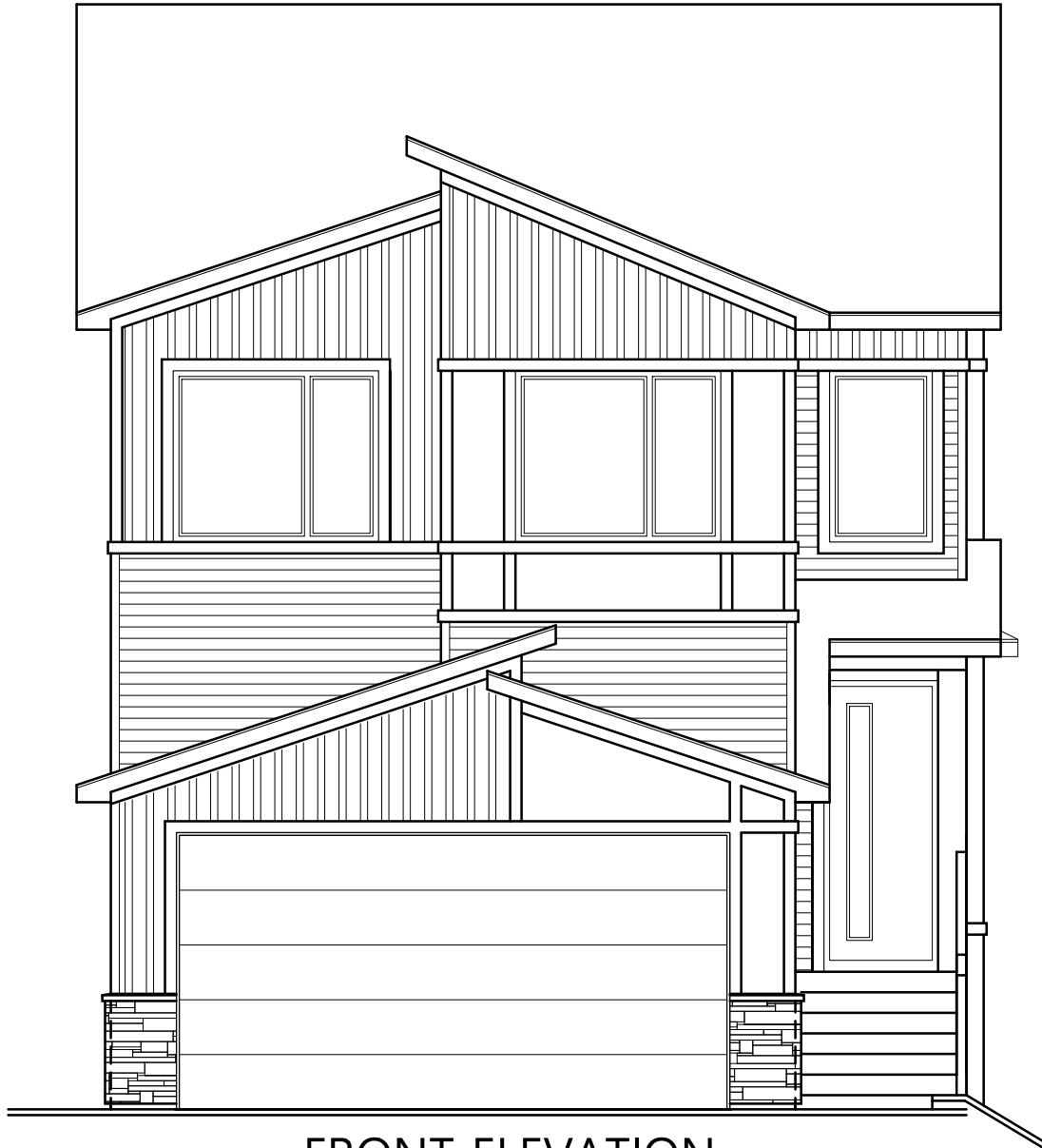
FRONT ELEVATION
