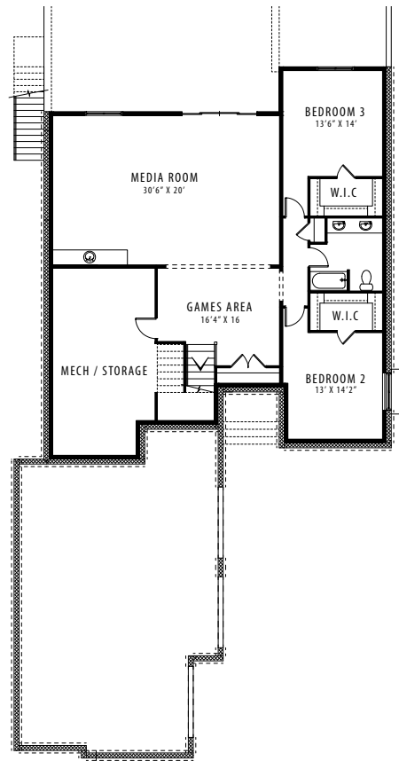
UPPER FLOOR | 1064 SQFT
